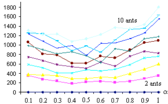
Figure 4: Number of evaluations per accentuation of probabilities for the 1-dimensional Rastrigin function.
