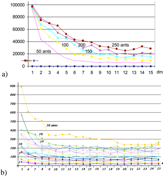
Figure 2: Number of evaluations per neighborhood radius for the 1-dimensional Rastrigin function: a) 50 to 250 ants and b) 2 to 30 ants.
