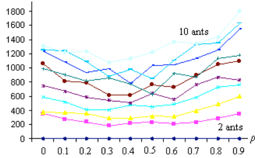
Figure 3: Number of evaluations per evaporation rate for the 1-dimensional Rastrigin function.
