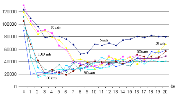
Figure 6: Number of evaluations per neighborhood radius for the tripod function: 5 to 500 ants.
