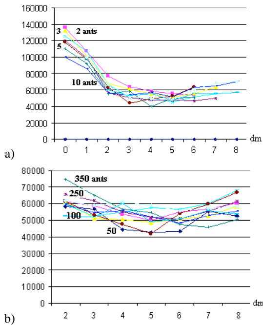
Figure 8: Number of evaluations per neighborhood radius for the 7 \times 7 f_{gauss} function: a) 2 to 10 ants and b) 50 to 500 ants.
